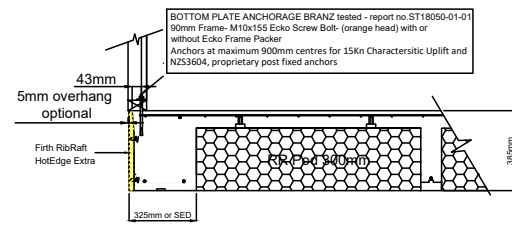
① 300mm FIRTH RIBRAFT POLYPOD 90mm WALL FRAME HOTEDGE EXTRA FIRTH RAFTMIX 20 OR 25MPa
