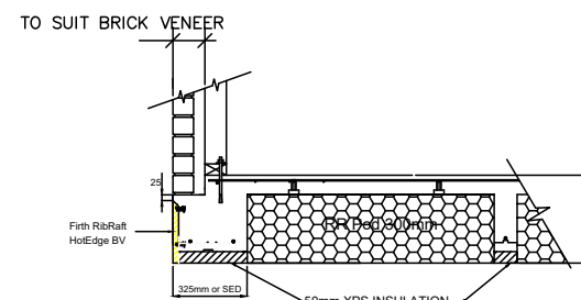
⑪ 300mm FIRTH RIBRAFT POLYPOD BRICK VENEER HOTEDGE WITH XPS INSULATION IN BEAMS & RIBS FIRTH RAFTMIX 20 OR 25MPa
