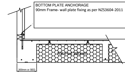
④ 300mm FIRTH RIBRAFT POLYPOD 90mm WALL FRAME FIRTH RAFTMIX 20 OR 25MPa
