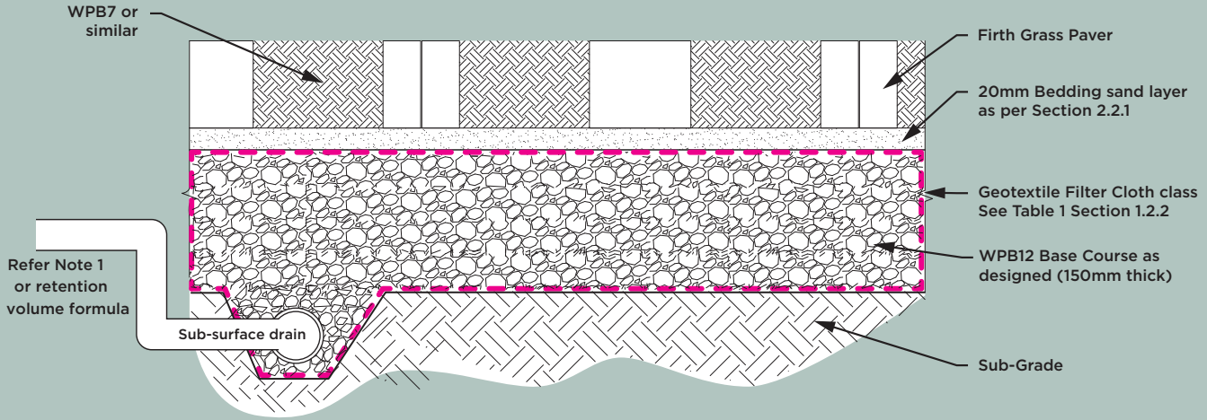
1.2.6 Installation Cross section drawing Firth Grass Paver 80mm
