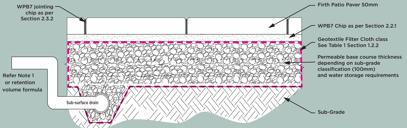
1.2.8 Installation Cross section drawing Firth Patio Paver 50mm
