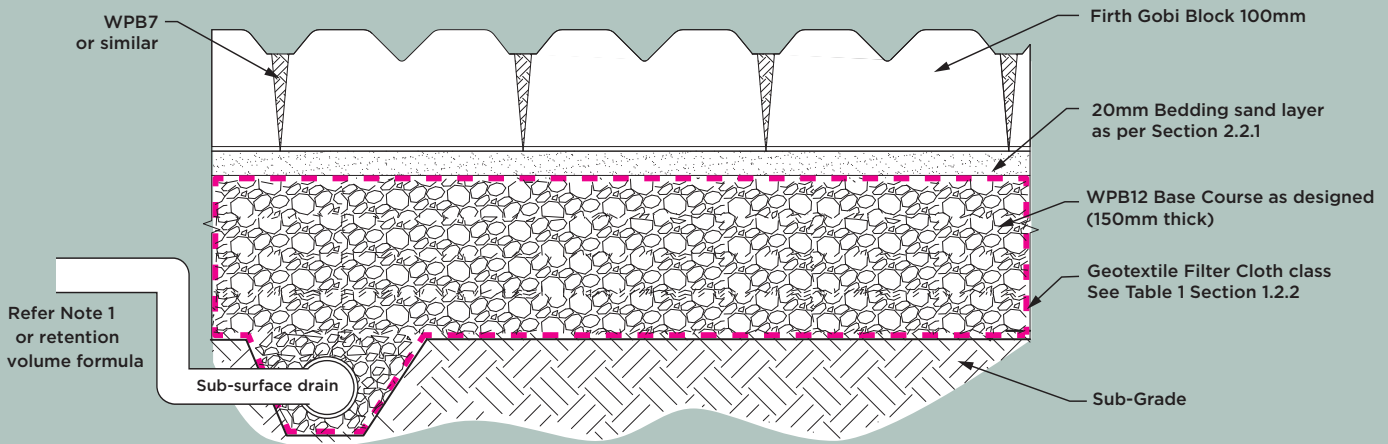
1.2.7 Installation Cross section drawing Firth Gobi® Block 100mm
